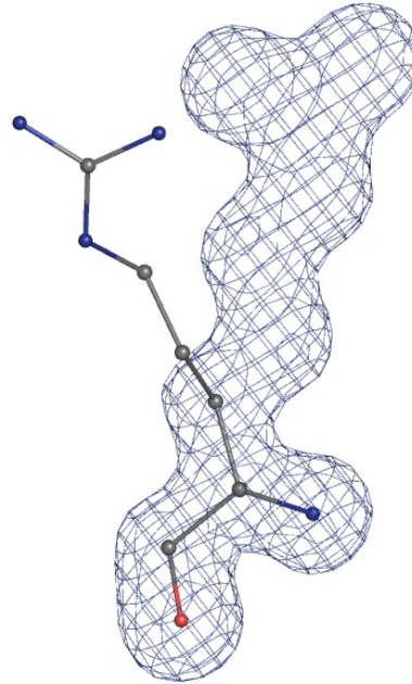
Simulated Annealing
